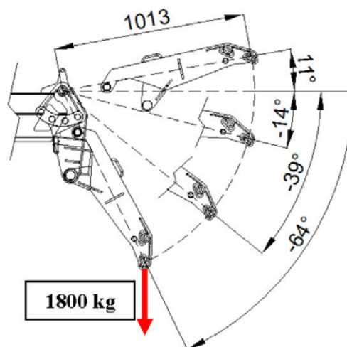
JIB1800-700.2M Short configuration
