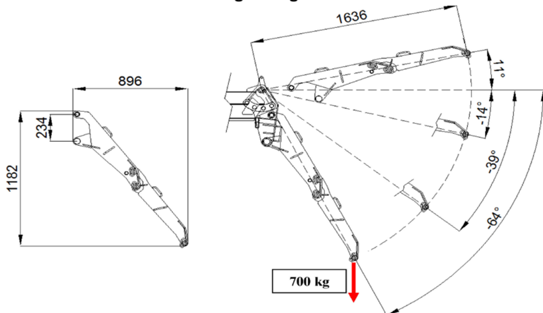
JIB1800-700.2M Long configuration
